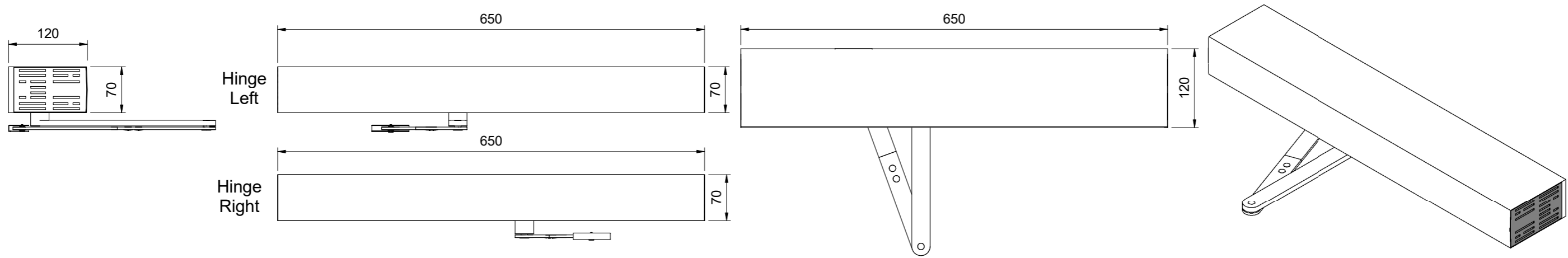
02 Side View 1 : 6
